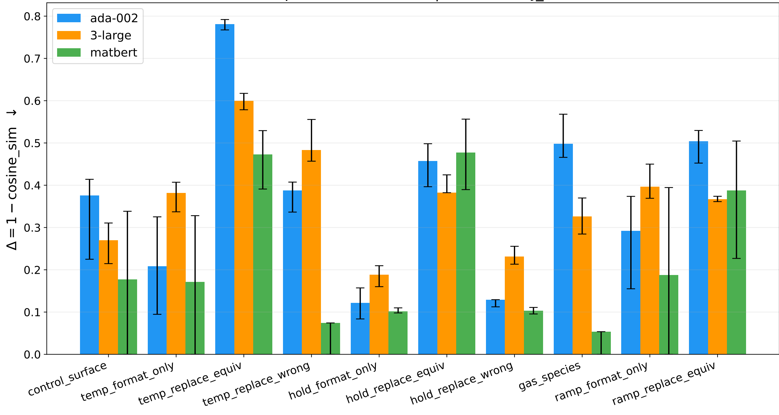
Group mean \Delta with IQR | Mode: PROJ_both
